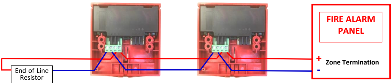
TYPICAL TERMINATION DIAGRAM (Using Terminal 1,2 and 3,4)
