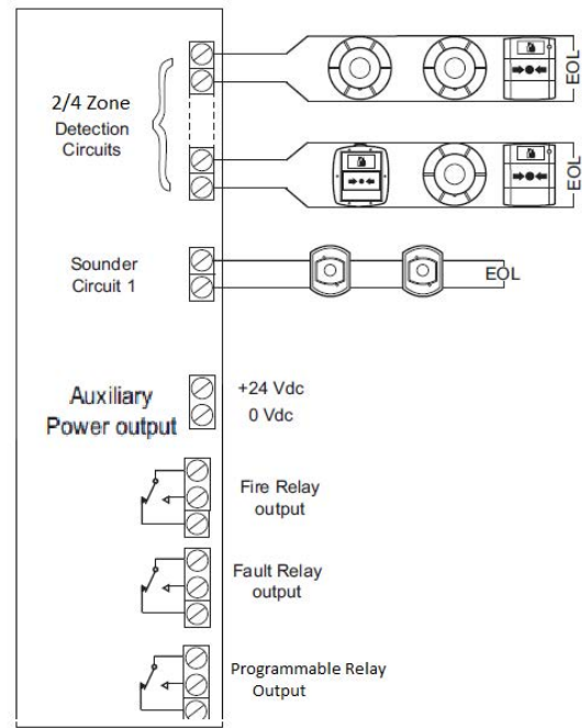
Circuit diagram*
